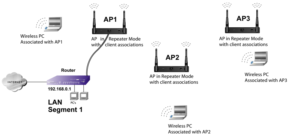
Figure 5-6: Multi-Point bridging
