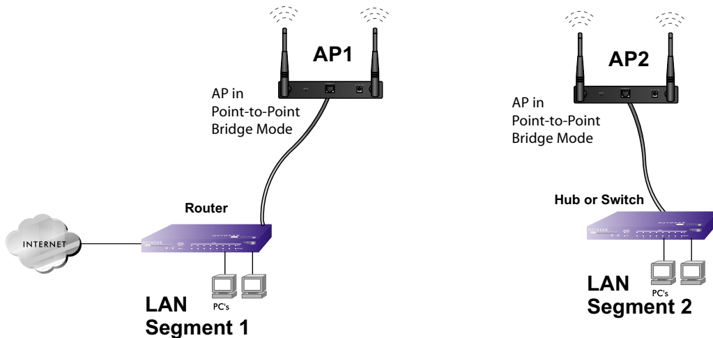
Figure 5-4: Point-to-Point Bridge
